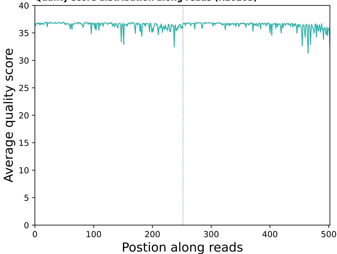
Quality score distribution along reads (R10205)
